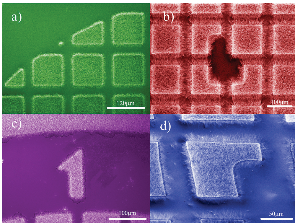
Figure 2. Demonstration of well-defined patterned growth of BNNTs on a substrate. (Artificial color was added to the SEM images.)
